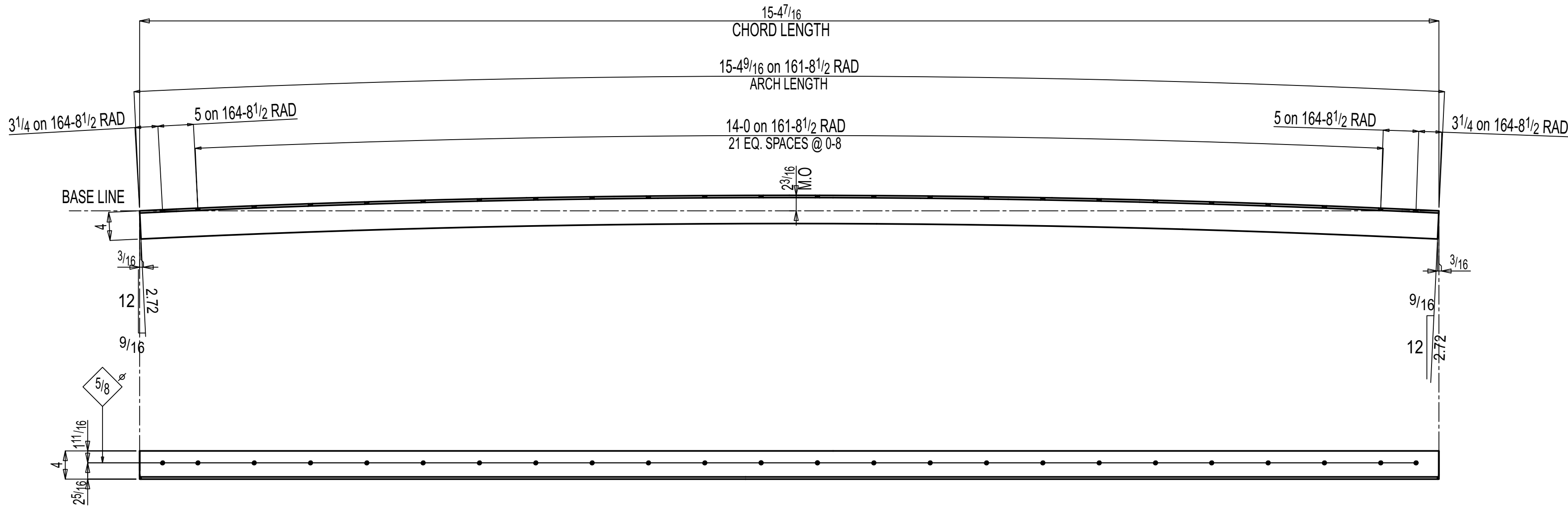
ONE ANGLE F-11.07A2
