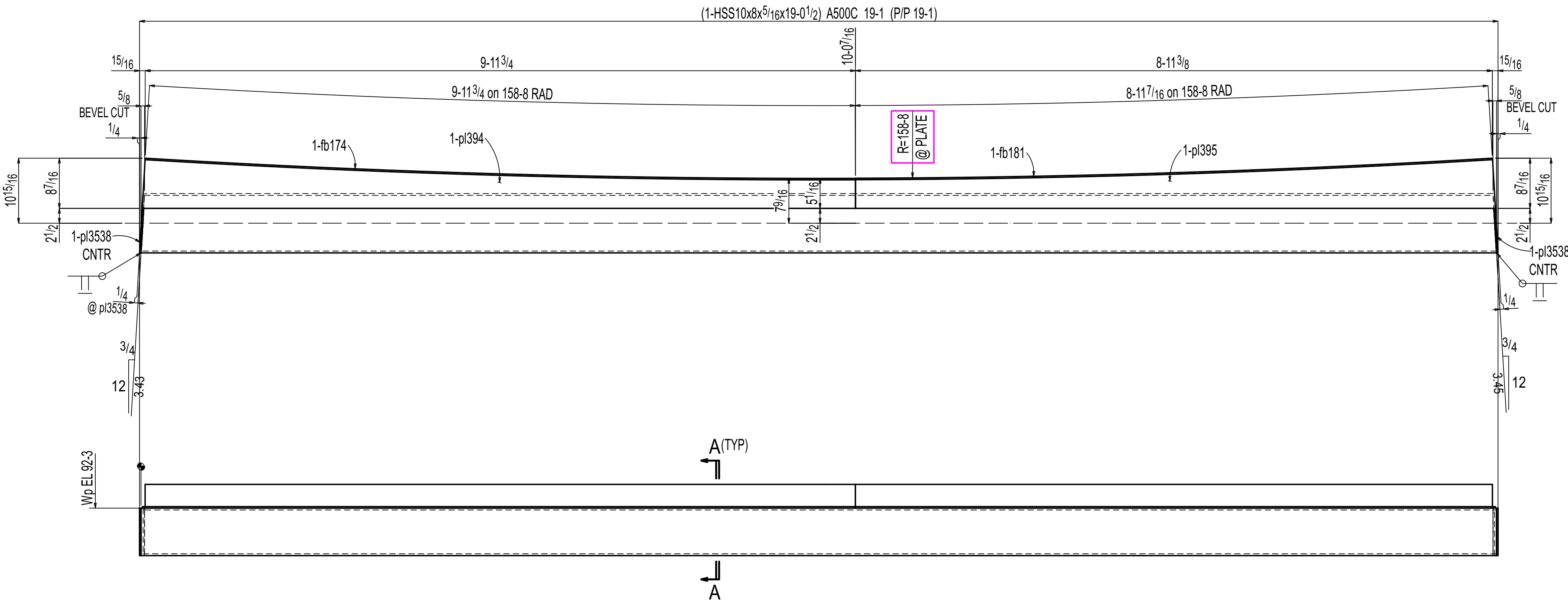
ONE BEAM F-11.05B2
