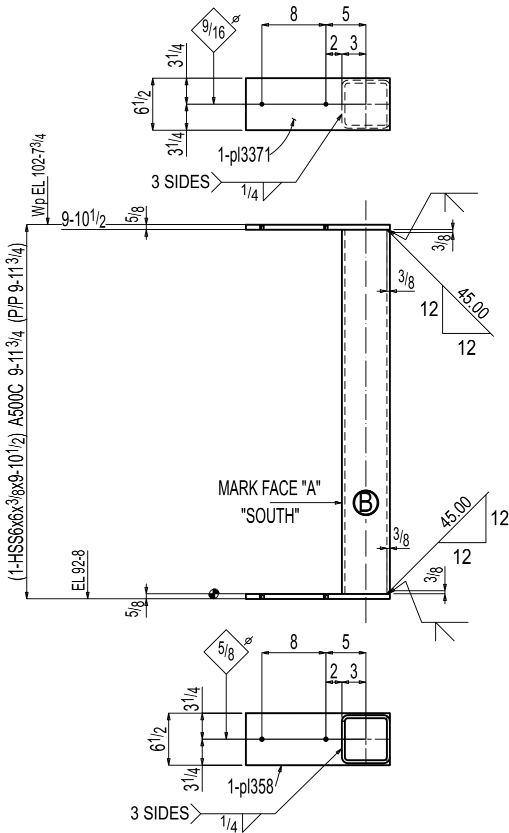
ONE COLUMN F-11.04C2
