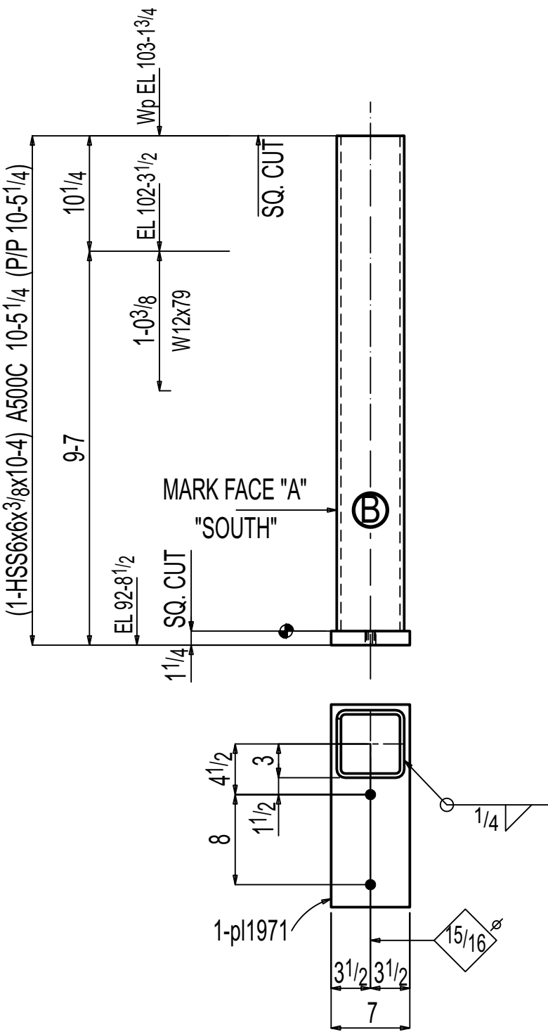
ONE COLUMN F-11.04C1
