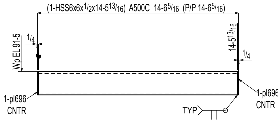
ONE BEAM F-11.07B1
