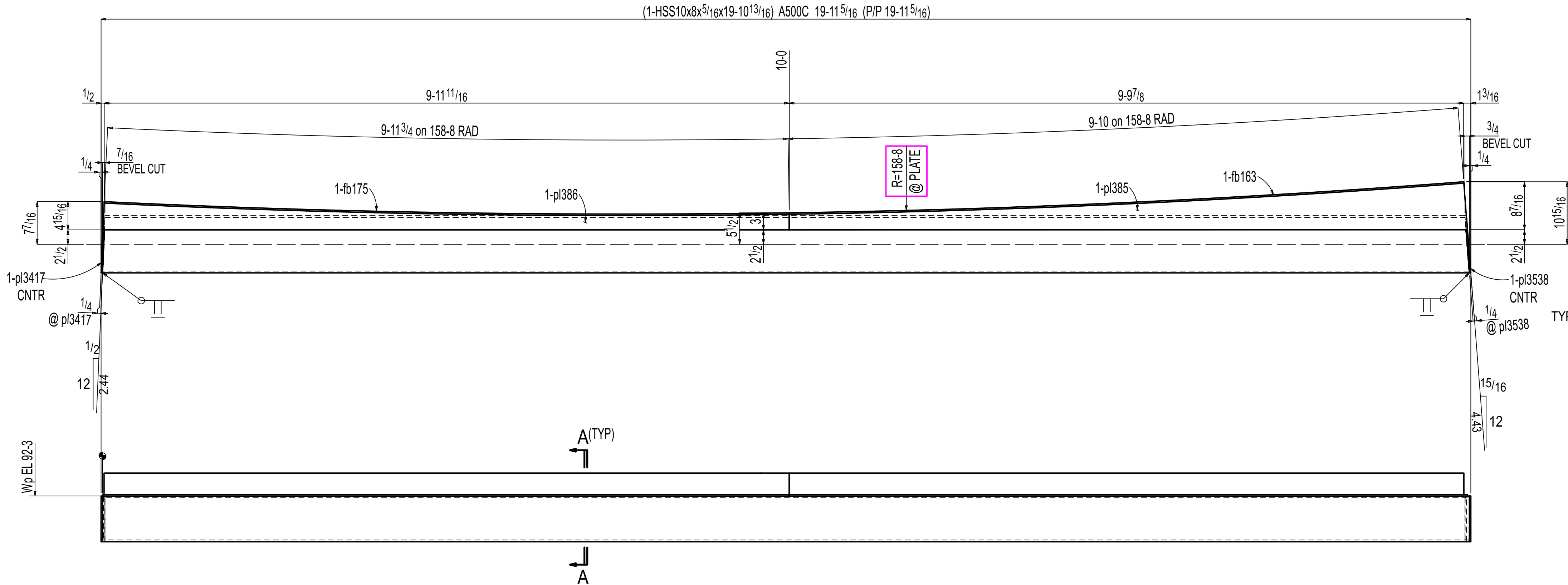
ONE BEAM F-11.05B1
