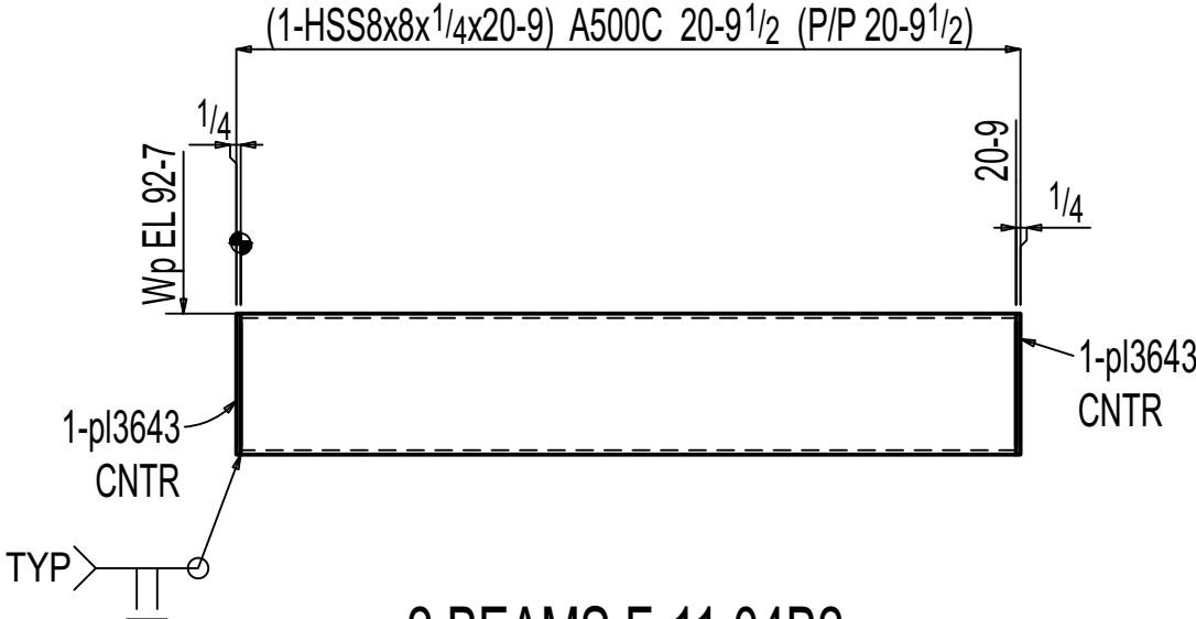
2 BEAMS F-11.04B2
