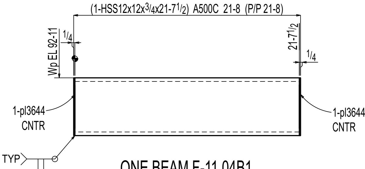
ONE BEAM F-11.04B1
